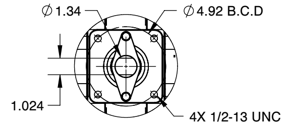
MOUNTING DIMENSIONS
