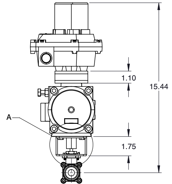
MOUNTING DIMENSIONS
