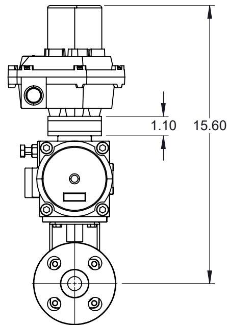
MOUNTING DIMENSIONS
