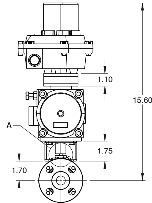
MOUNTING DIMENSIONS
