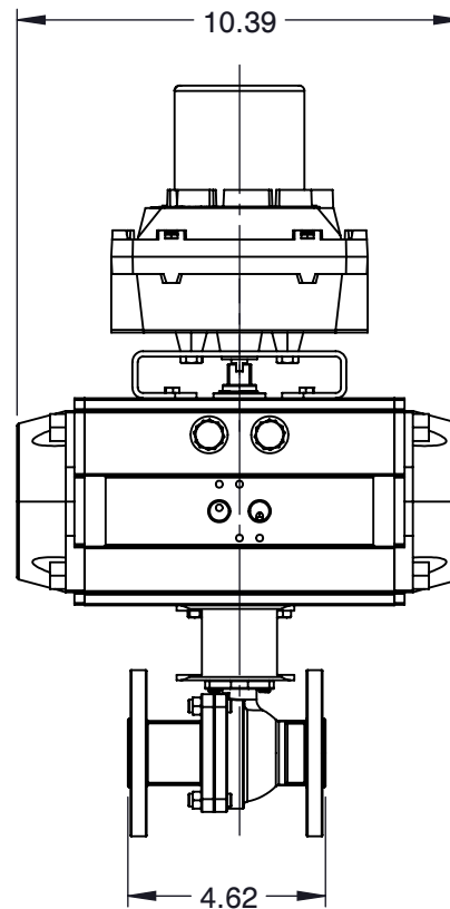
DETAIL A
