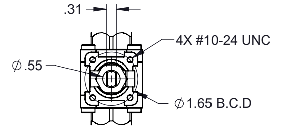
MOUNTING DIMENSIONS
