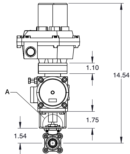
MOUNTING DIMENSIONS
