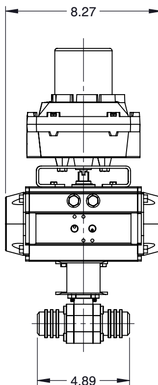
DETAIL A
