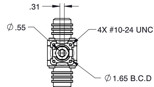
MOUNTING DIMENSIONS
