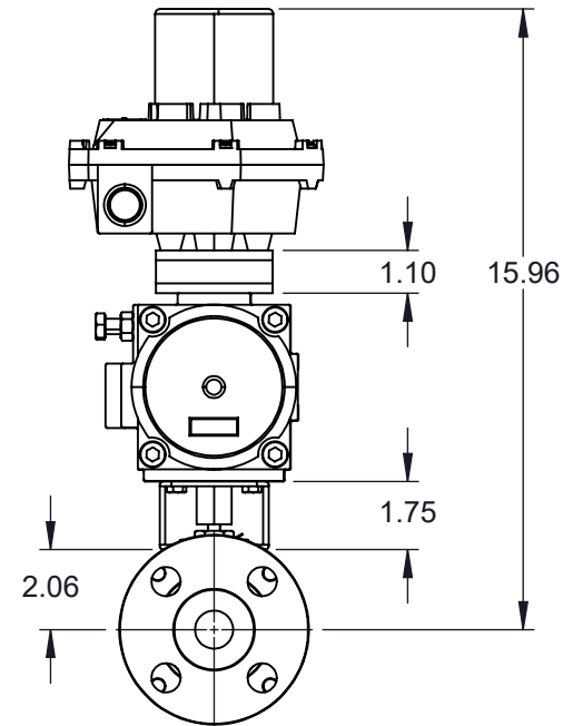
MOUNTING DIMENSIONS
