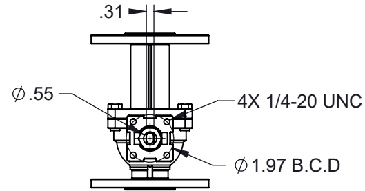
MOUNTING DIMENSIONS
