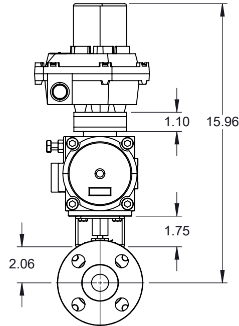
MOUNTING DIMENSIONS
