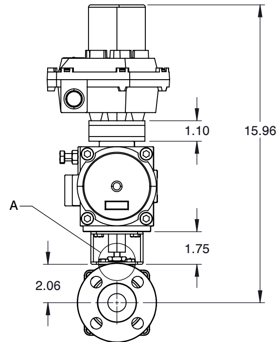
MOUNTING DIMENSION
