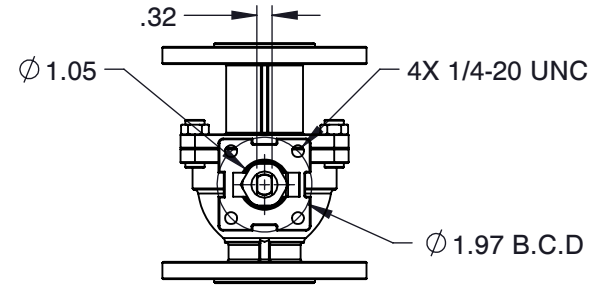
MOUNTING DIMENSION
