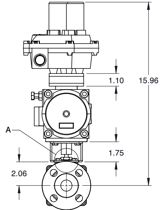
MOUNTING DIMENSION
