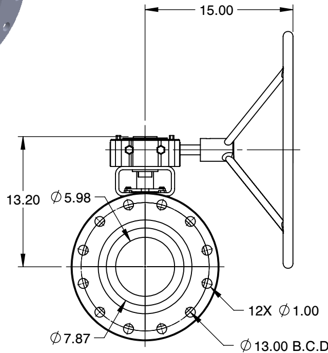
DETAIL C
