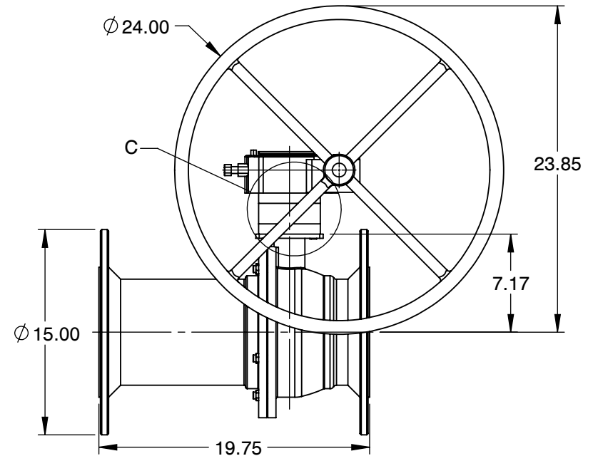
MOUNTING DIMENSIONS
