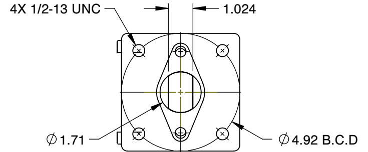
MOUNTING DIMENSIONS
