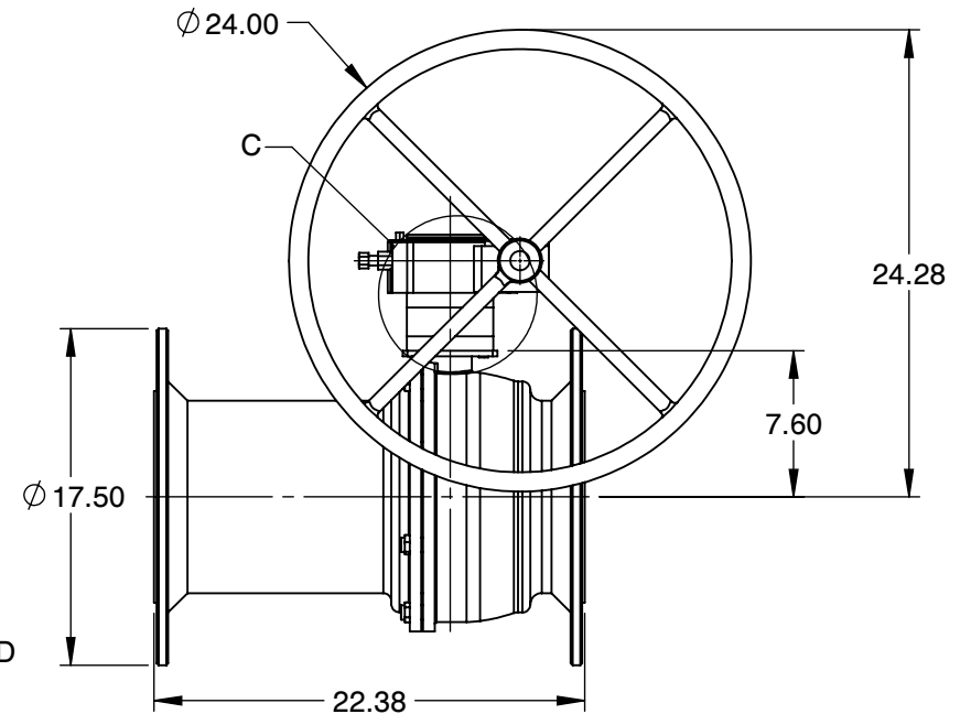
MOUNTING DIMENSIONS
