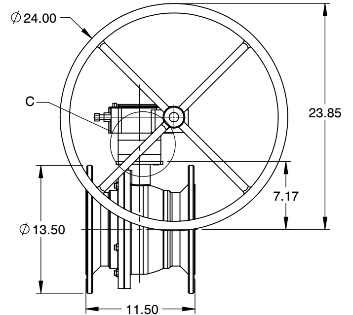
MOUNTING DIMENSIONS
