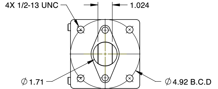
MOUNTING DIMENSIONS
