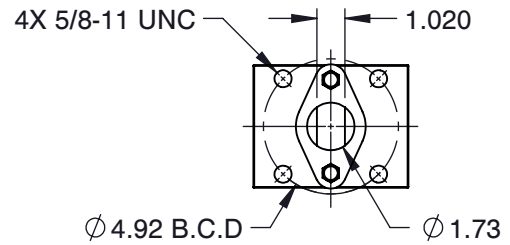
MOUNTING DIMENSIONS
