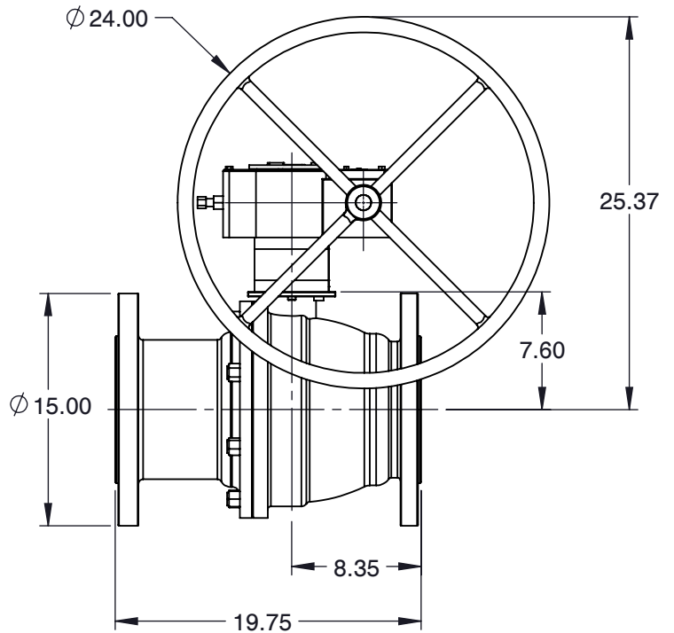
MOUNTING DIMENSIONS
