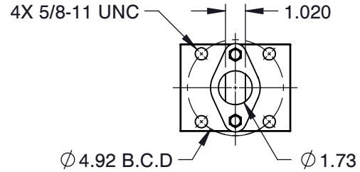
MOUNTING DIMENSIONS
