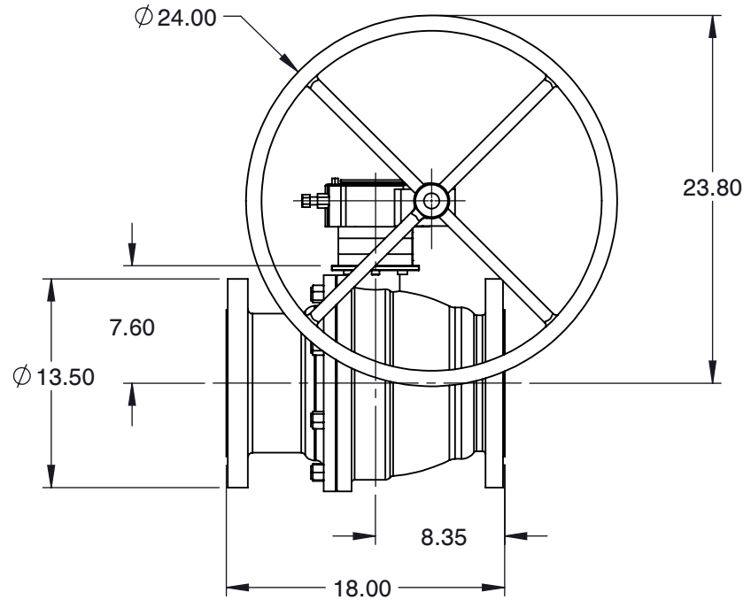
MOUNTING DIMENSIONS
