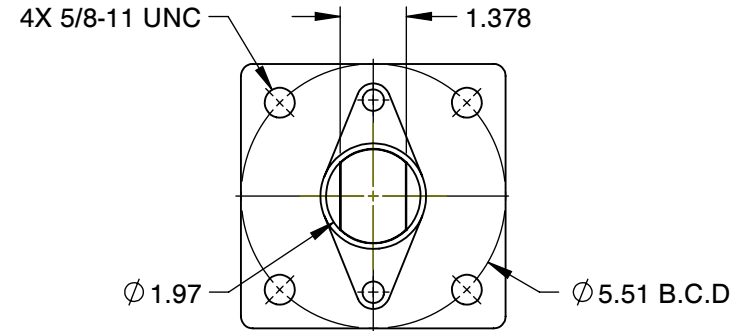
MOUNTING DIMENSIONS
