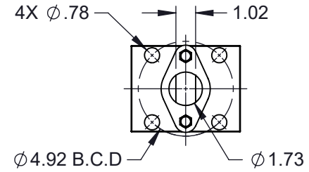
MOUNTING DIMENSIONS
