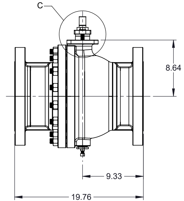
MOUNTING DIMENSIONS
