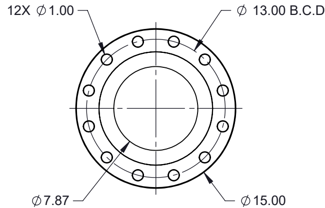
FLANGE DETAILS
