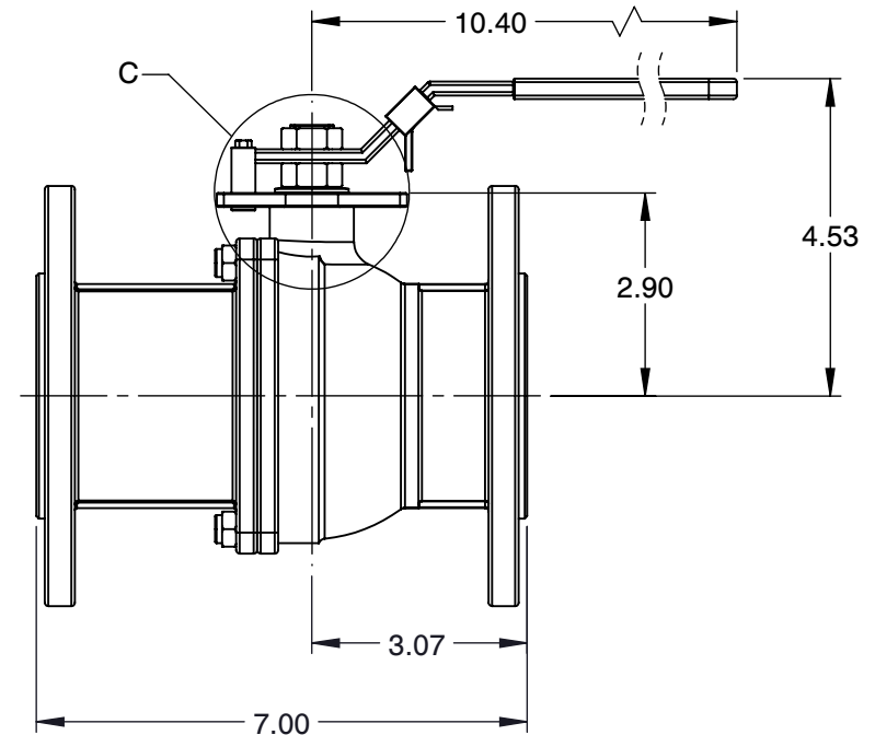
MOUNTING DIMENSIONS
