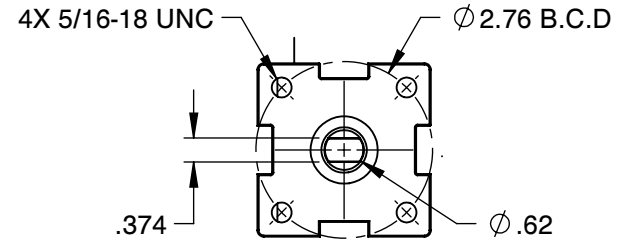
MOUNTING DIMENSIONS
