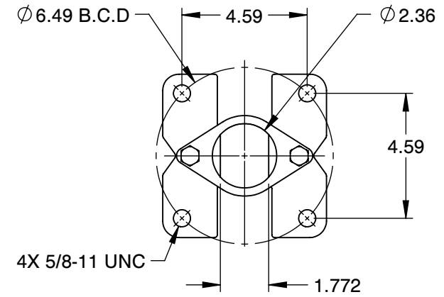
MOUNTING DIMENSIONS
