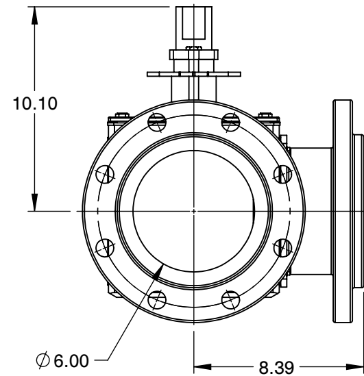
MOUNTING DIMENSIONS
