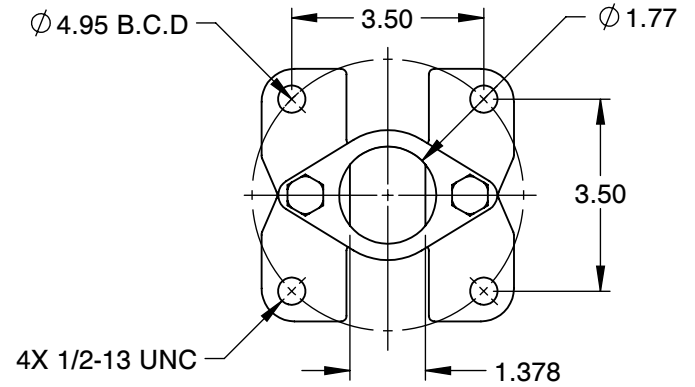
MOUNTING DIMENSIONS
