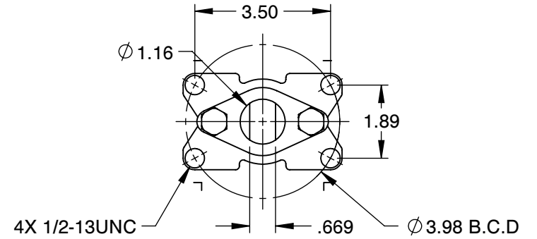
MOUNTING DIMENSIONS
