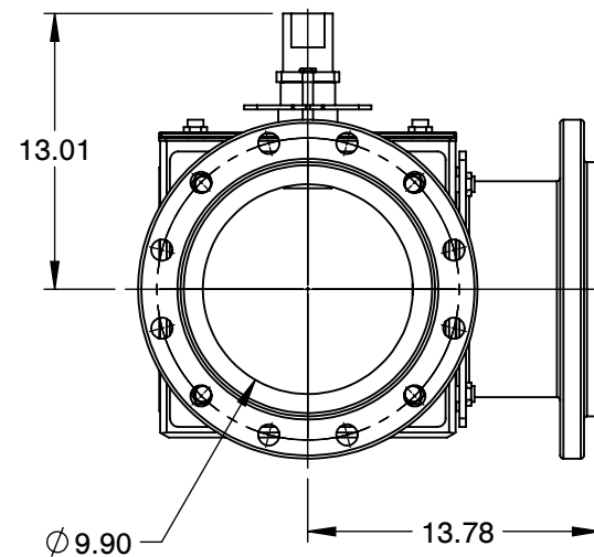
MOUNTING DIMENSIONS
