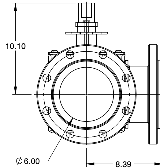
MOUNTING DIMENSIONS
