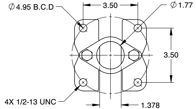
MOUNTING DIMENSIONS
