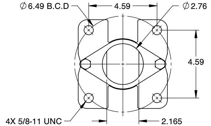
MOUNTING DIMENSIONS
