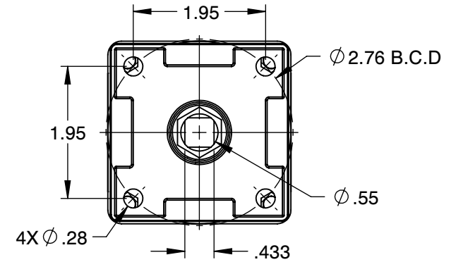
MOUNTING DIMENSIONS
