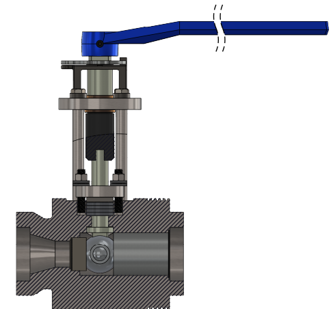
SECTION VIEW
