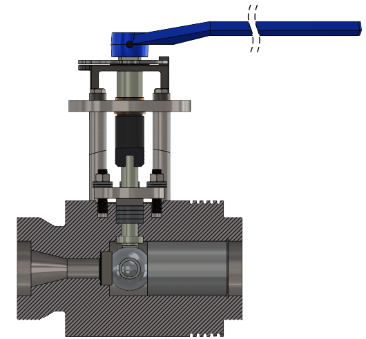
SECTION VIEW
