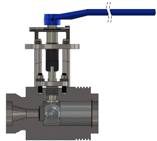
SECTION VIEW
