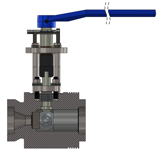
SECTION VIEW
