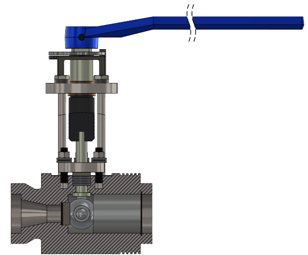
SECTION VIEW
