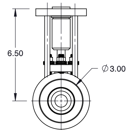
SECTION VIEW
